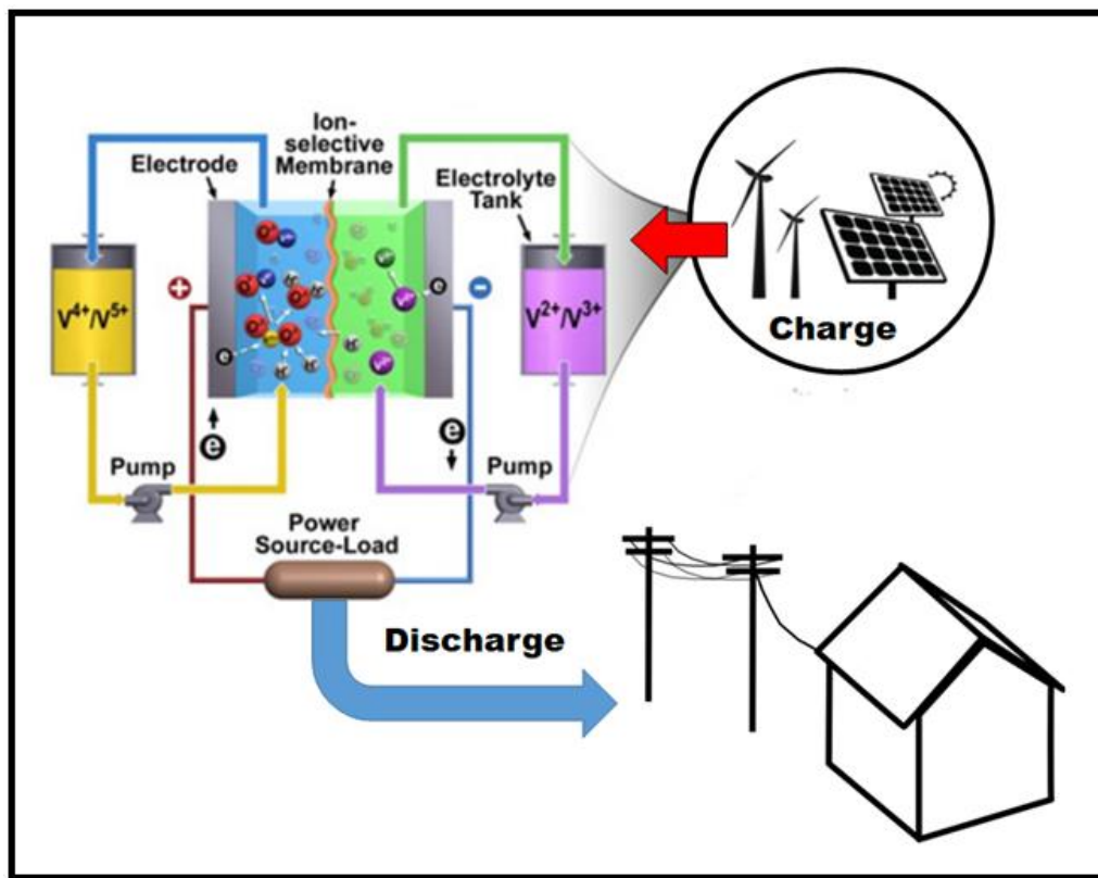
Figure 3: Vanadium Redox Flow Battery
